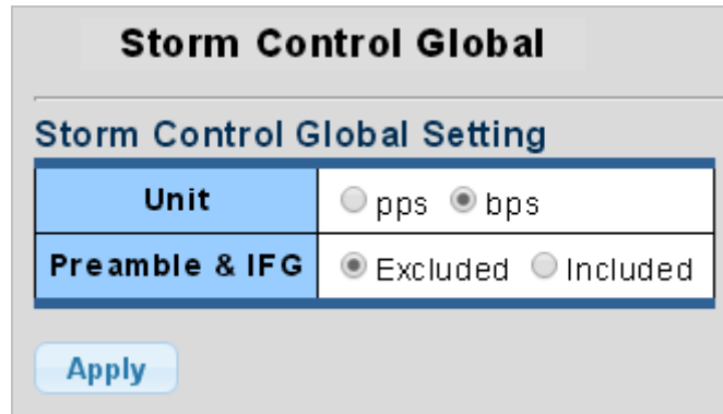
Figure 4-9-71 Storm Control Global Setting Page Screenshot
