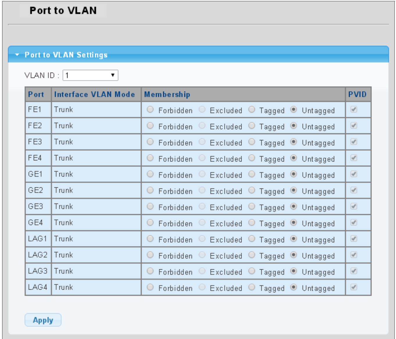
Figure 4-5-7 Port to VLAN Setting Page Screenshot
