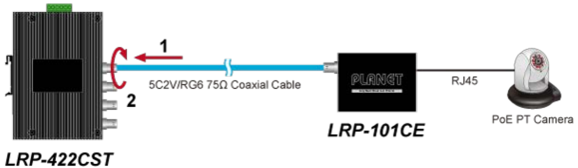
Figure 2-3 How to insert the coaxial cable from LRP Managed Switch
