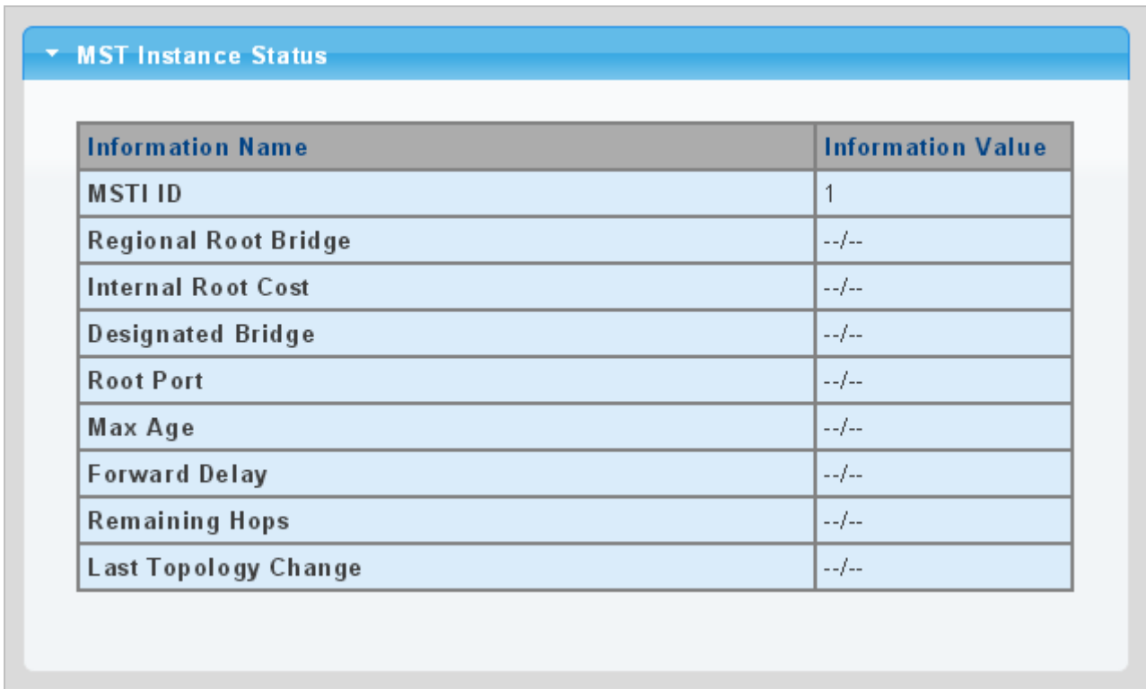
Figure 4-6-14 MST Instance Status Page Screenshot
