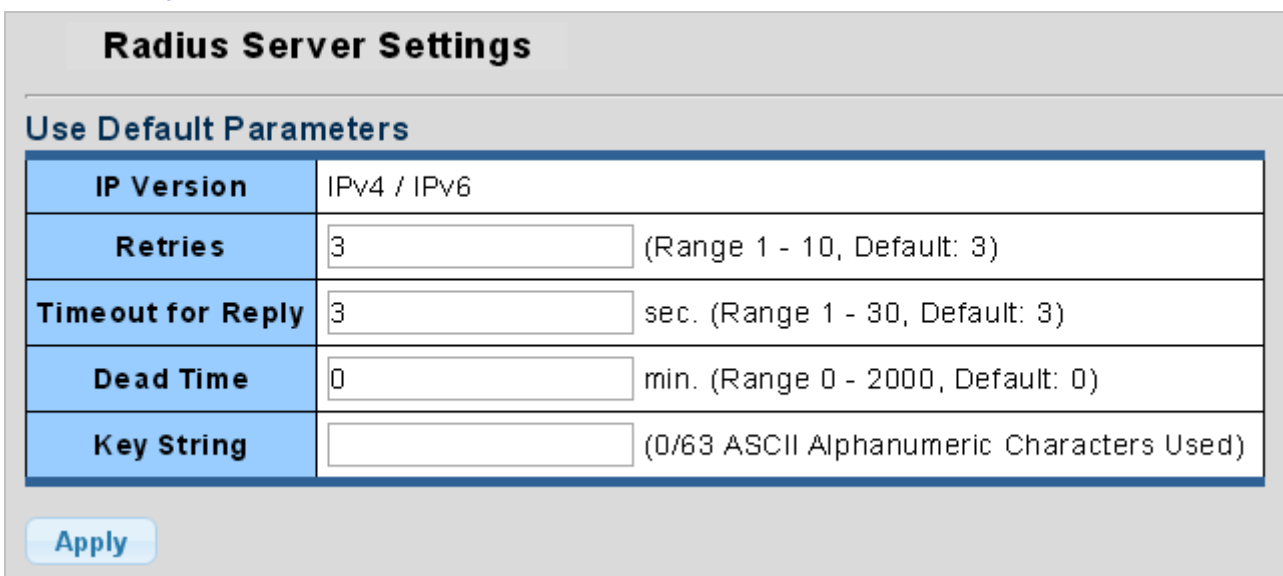
Figure 4-9-10 Use Default Parameters Page Screenshot
