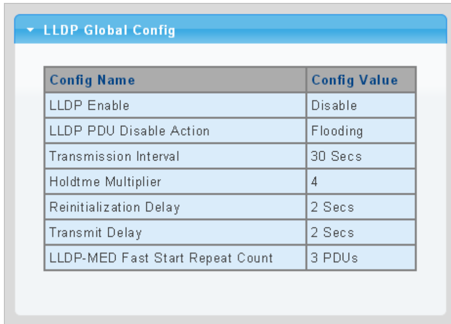
Figure 4-12-2 LLDP Global Config Page Screenshot
