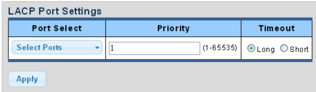
Figure 4-4-10 LACP Port Setting Page Screenshot
