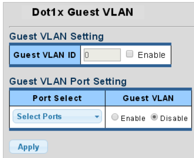
Figure 4-9-7 Guest VLAN Setting Page Screenshot
