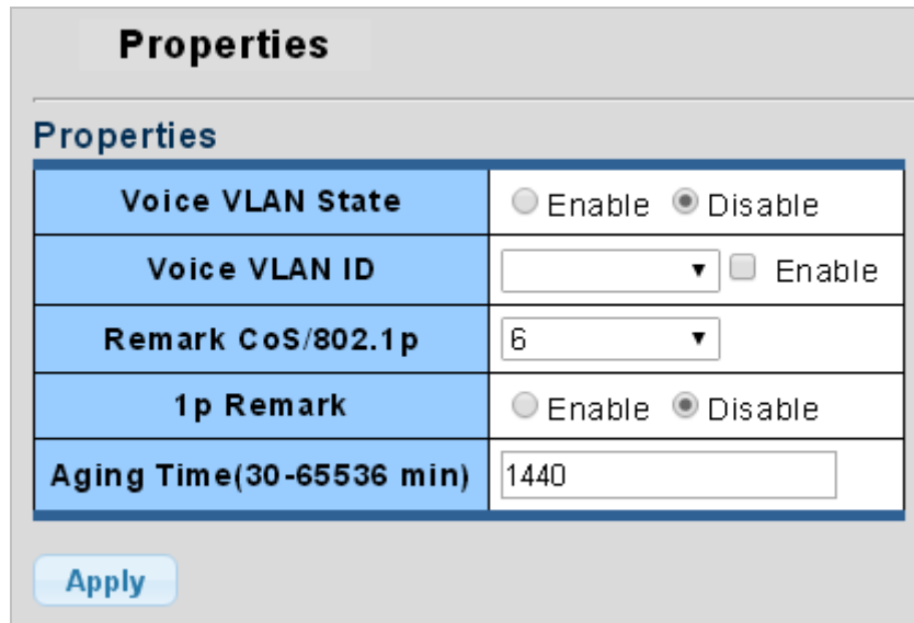
Figure 4-8-22 Properties Page Screenshot
