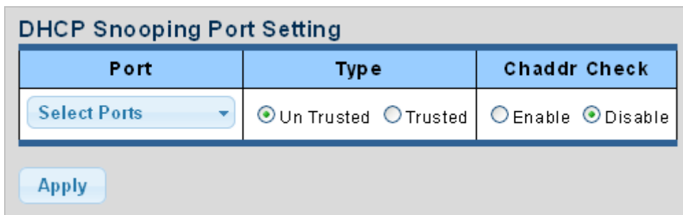
Figure 4-9-39 DHCP Snooping Port Setting Page Screenshot
