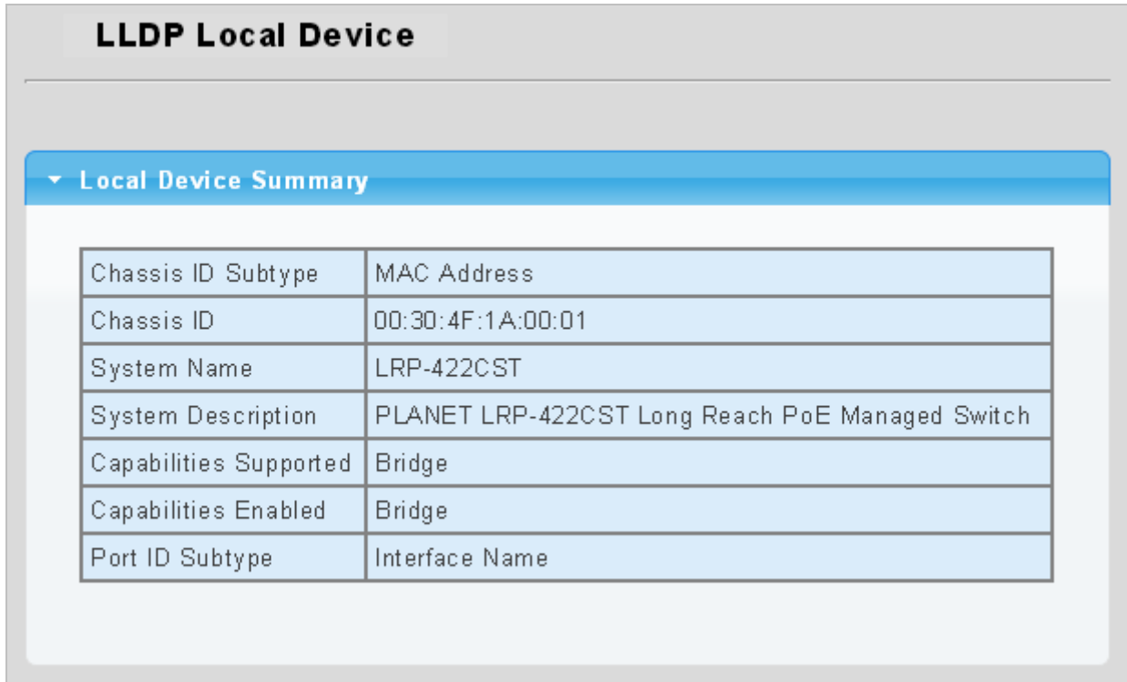
Figure 4-12-7 Local Device Summary Page Screenshot
