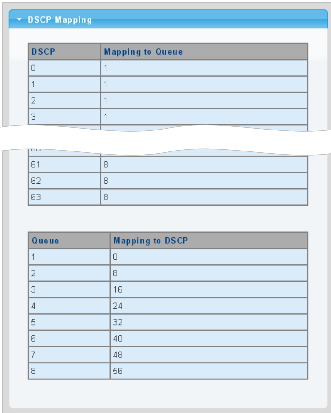
Figure 4-8-9 DSCP Mapping Page Screenshot
