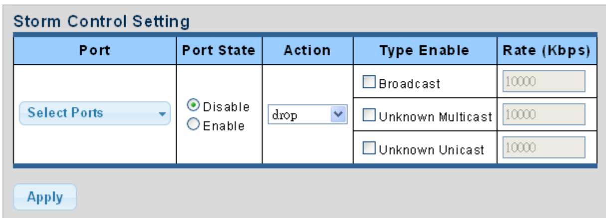
Figure 4-9-73 Storm Control Setting Page Screenshot
