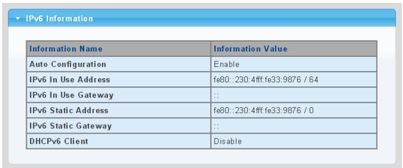
Figure 4-2-5 IPv6 Information Page Screenshot
