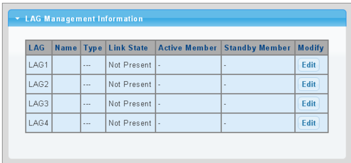
Figure 4-4-5 LAG Management Information Page Screenshot
