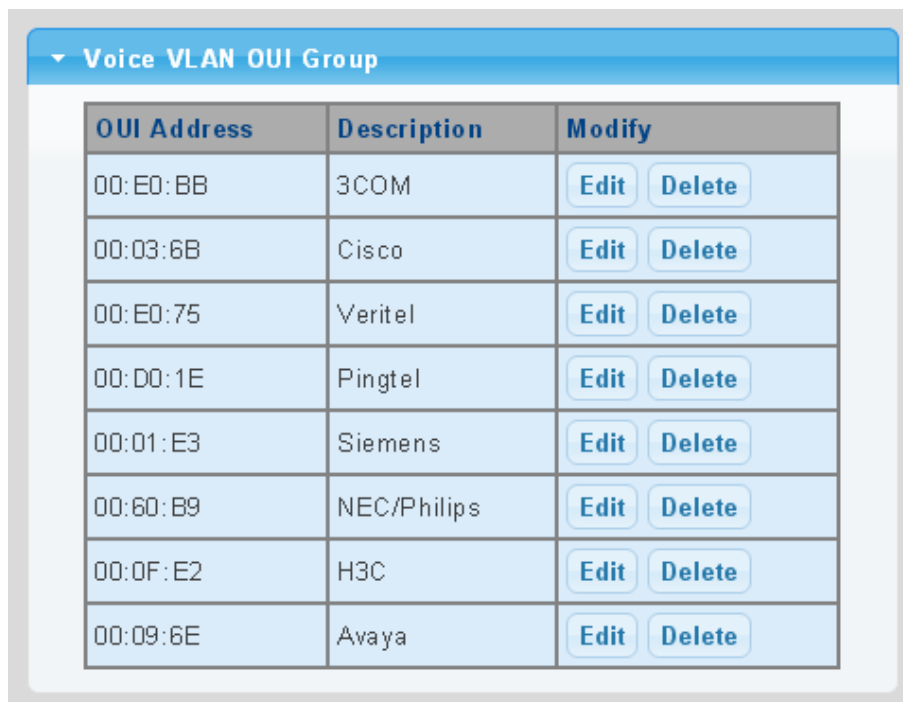
Figure 4-8-25 Voice VLAN OUI Group Page Screenshot
