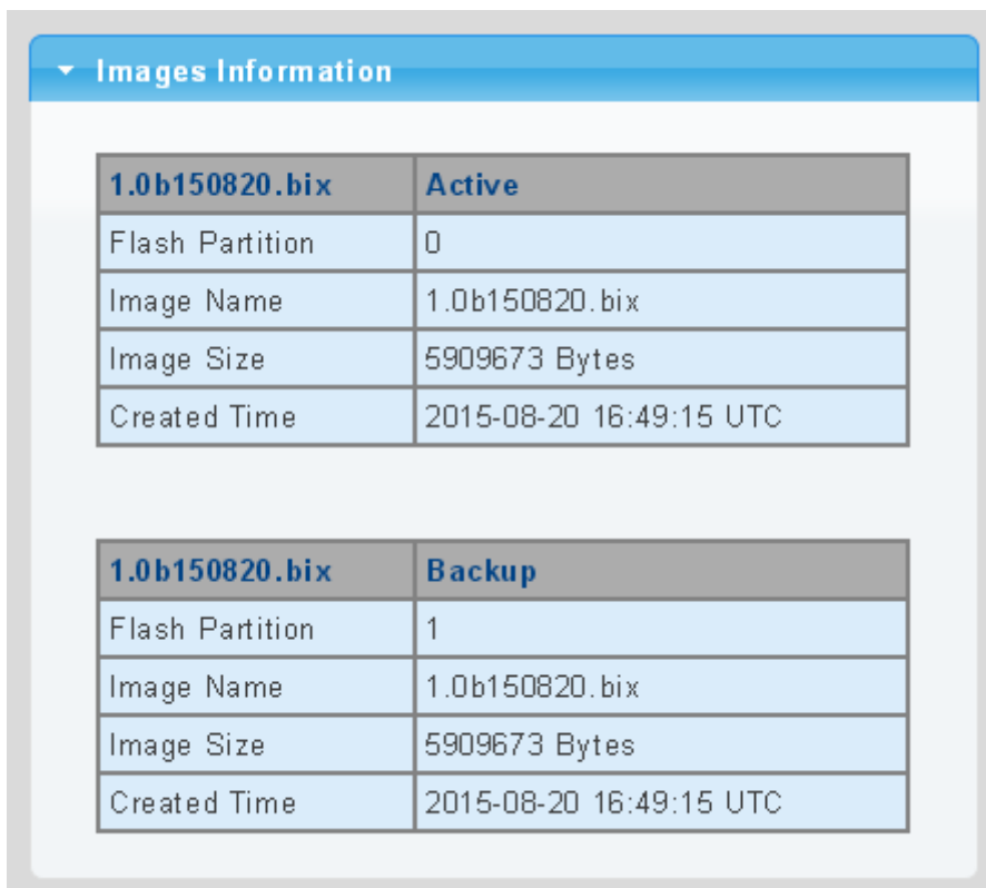
Figure 4-16-6: Dual Image Information Page Screenshot
