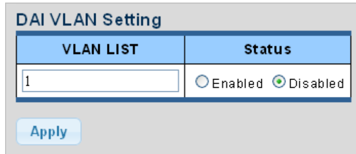
Figure 4-9-54 DAI VLAN Setting Page Screenshot
