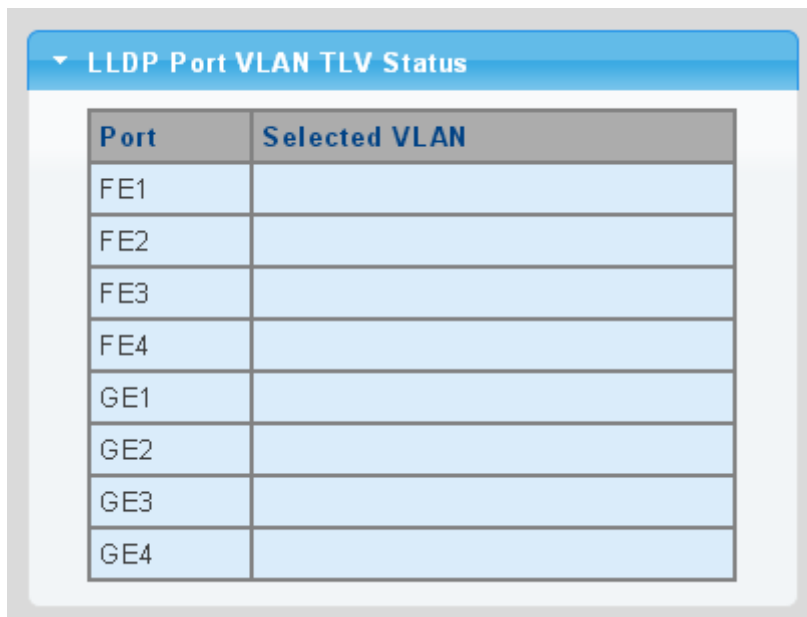
Figure 4-12-6 LLDP Port VLAN TLV Status Page Screenshot
