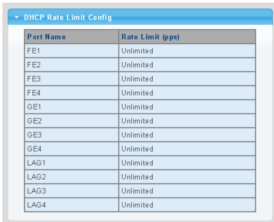
Figure 4-9-45 DHCP Rate Limit Setting Page Screenshot
