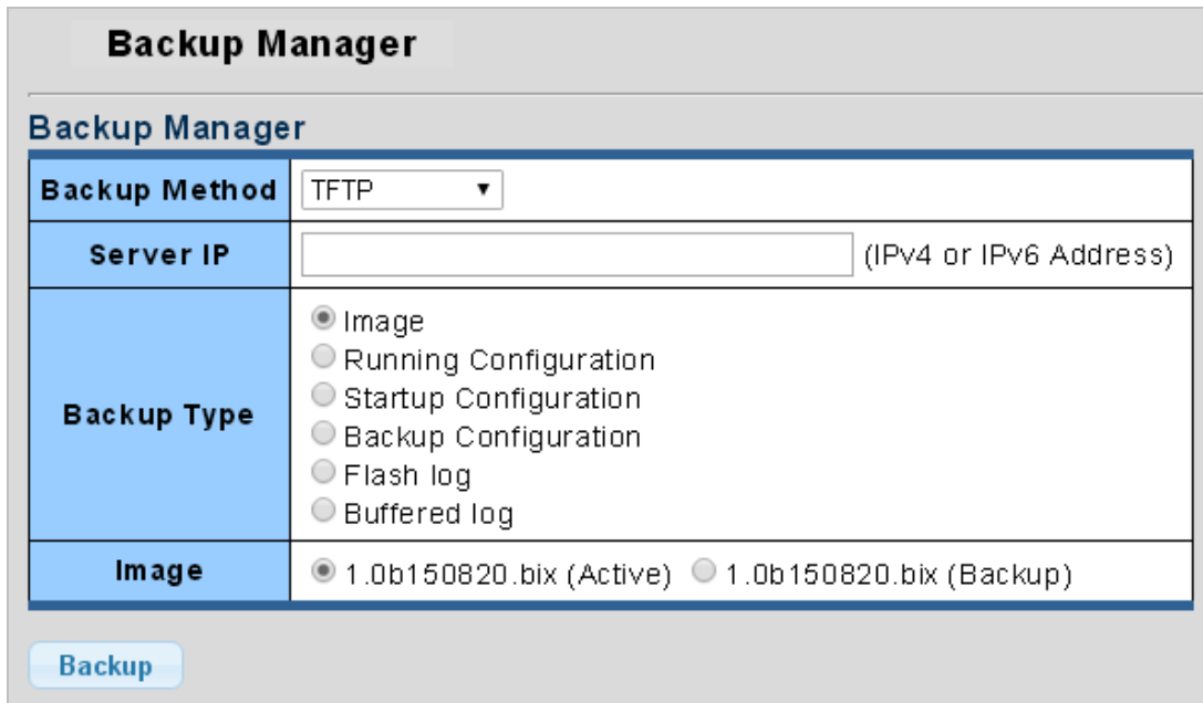
Figure 4-16-3 Backup Manager Page Screenshot
