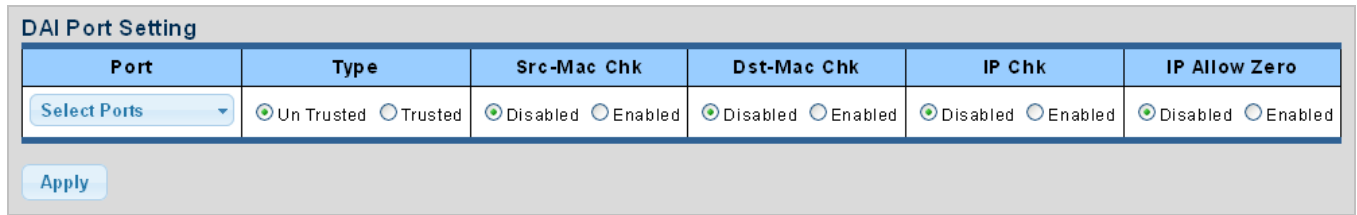
Figure 4-9-56 DAI Port Setting Page Screenshot
