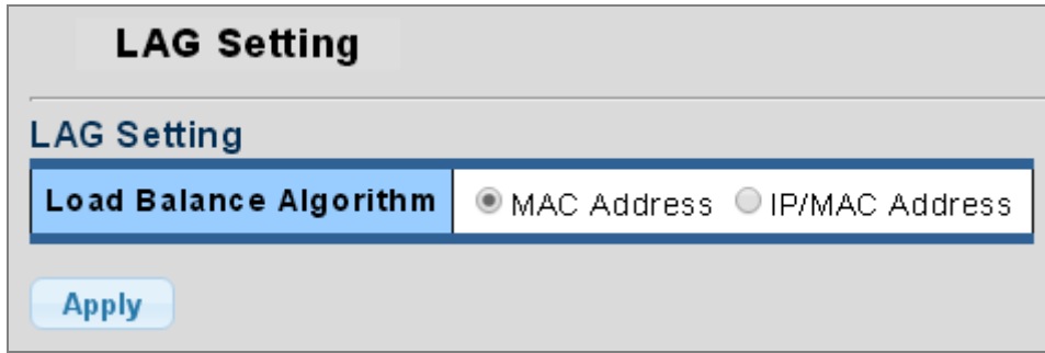
Figure 4-4-2 LAG Setting Page Screenshot
