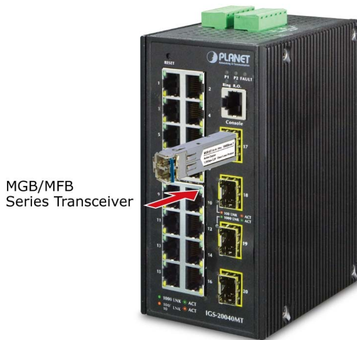
Figure 2-1 Plug in the SFP transceiver
