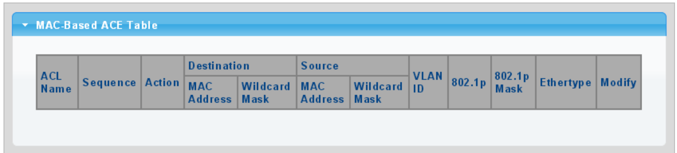
Figure 4-10-4 MAC-based ACE Table Page Screenshot
