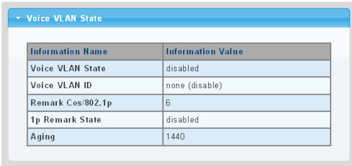
Figure 4-8-23 Properties Page Screenshot
