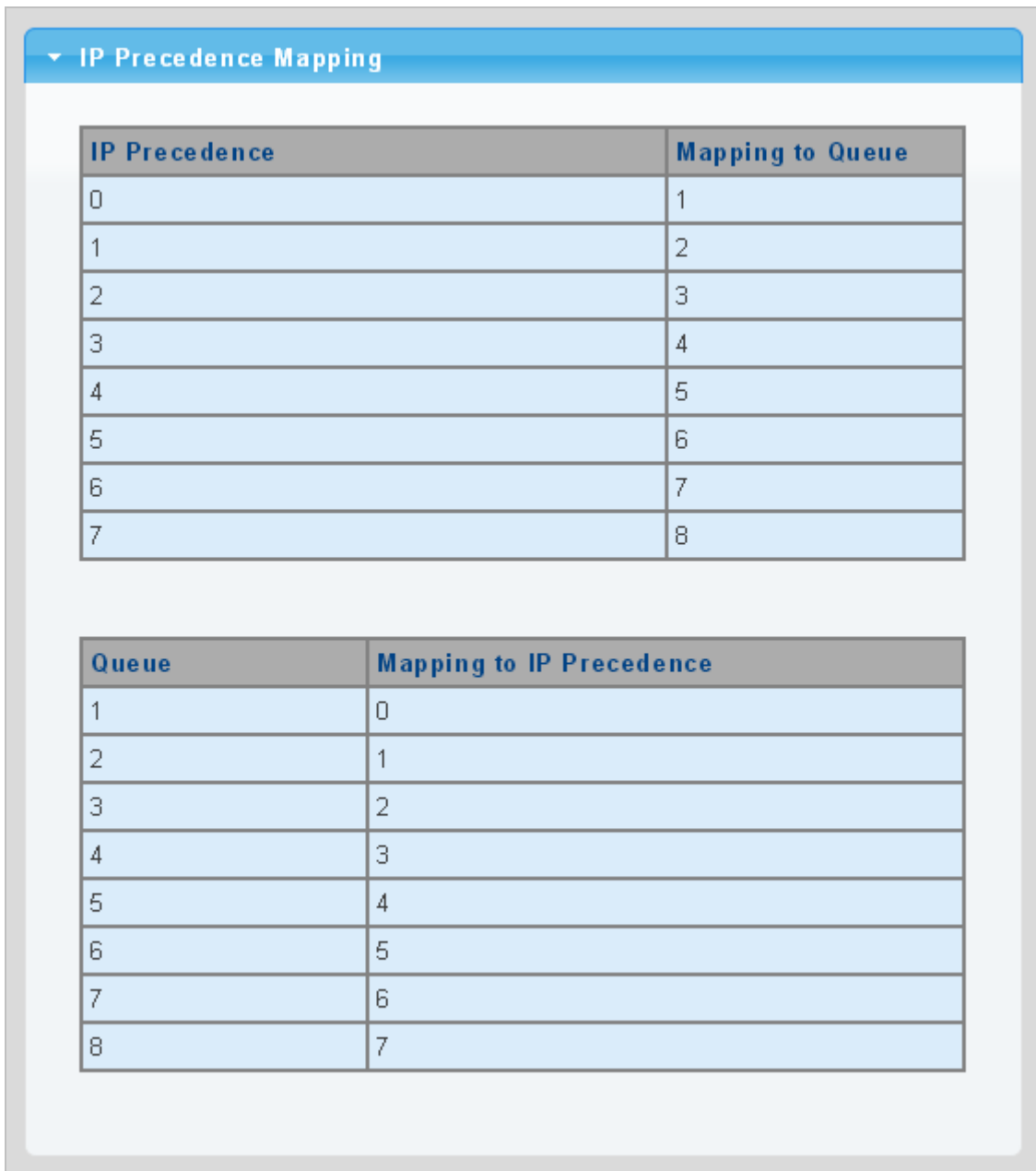
Figure 4-8-11 IP Precedence Mapping Page Screenshot
