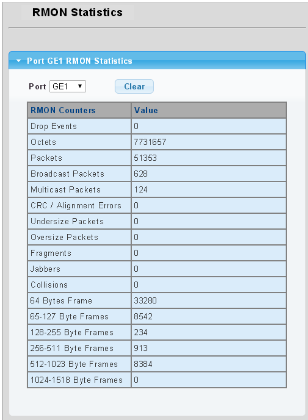
Figure 4-14-1: RMON Statistics Detail Page Screenshot
