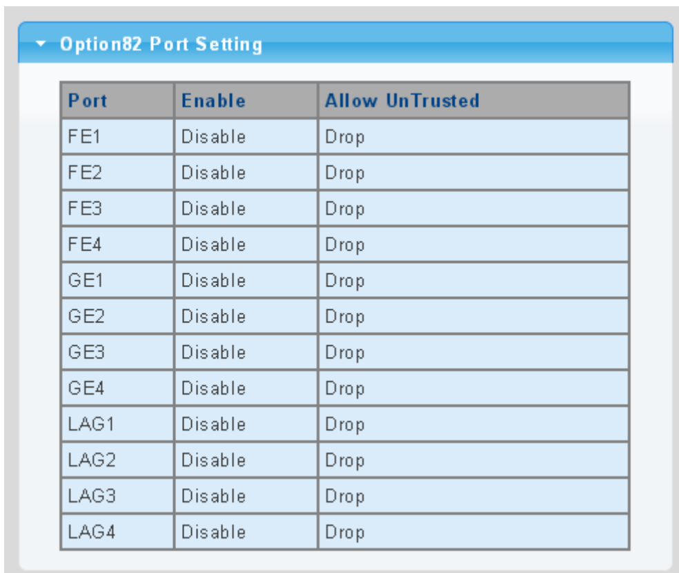
Figure 4-9-49 Option 82 Global Setting Page Screenshot
