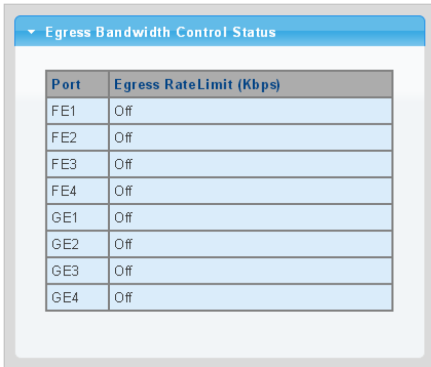
Figure 4-8-19 Egress Bandwidth Control Status Page Screenshot
