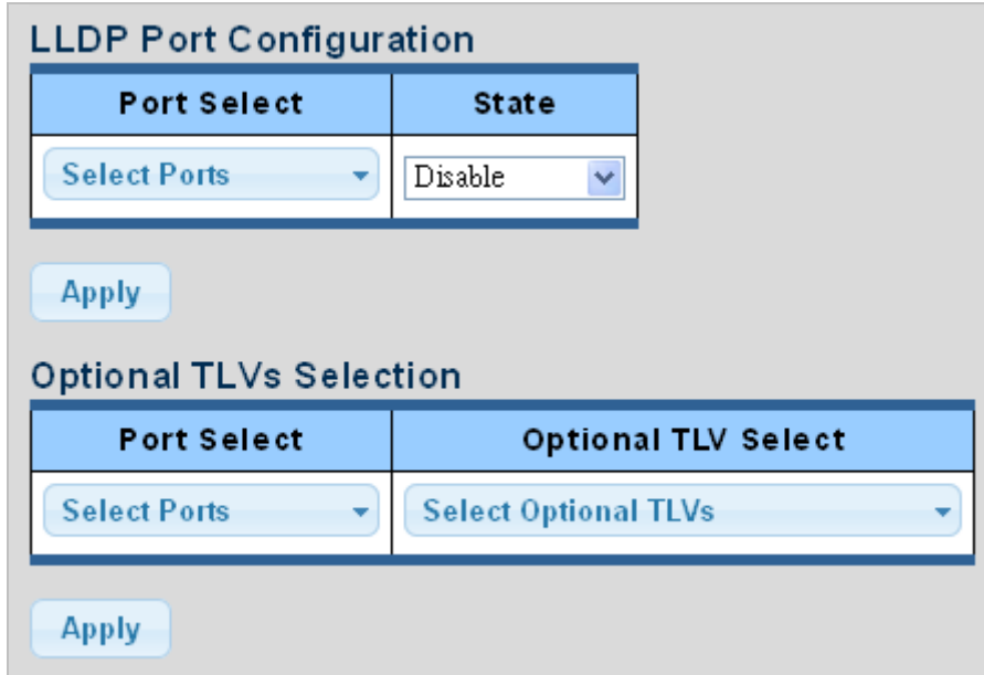
Figure 4-12-3 LLDP Port Configuration and Optional TLVs Selection Page Screenshot
