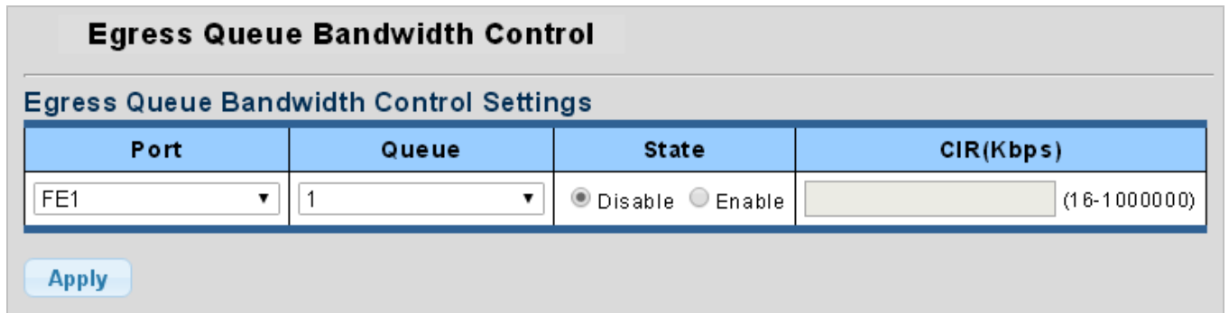
Figure 4-8-20 Egress Queue Bandwidth Settings Page Screenshot
