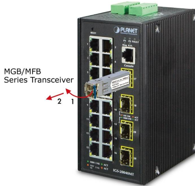
Figure 2-2 How to Pull Out the SFP Transceiver
