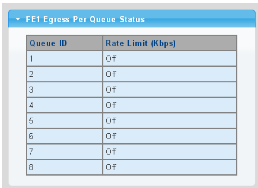
Figure 4-8-21 Egress Queue Status Page Screenshot
