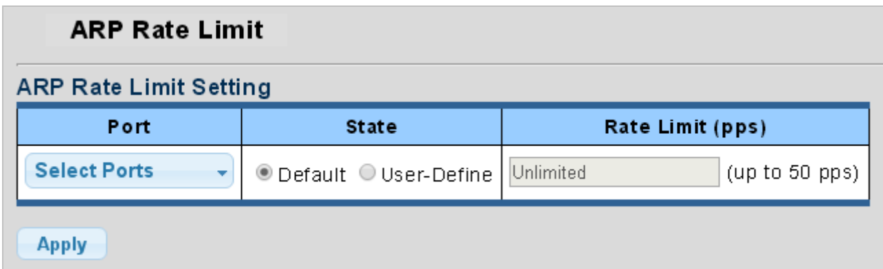
Figure 4-9-59 ARP Rate Limit Setting Page Screenshot
