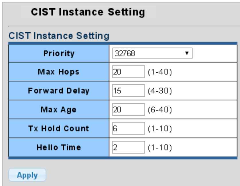
Figure 4-6-8: CIST Instance Setting Page Screenshot
