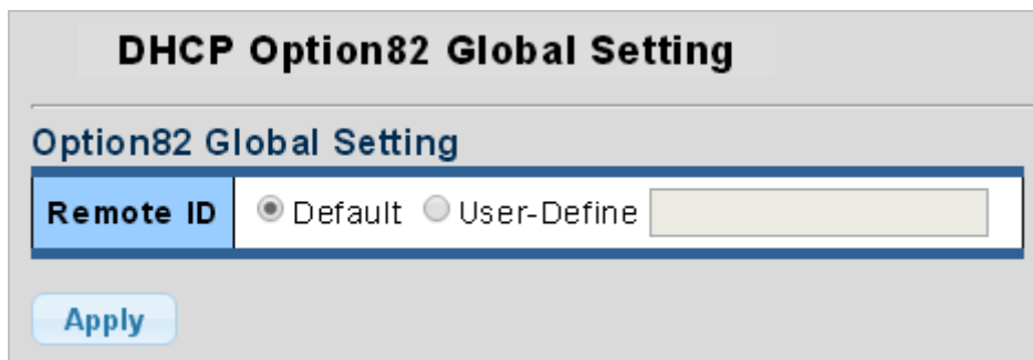
Figure 4-9-46 Option 82 Global Setting Page Screenshot
