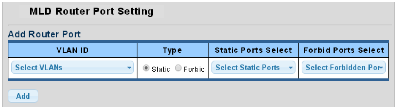
Figure 4-7-27 Add Router Port Page Screenshot
