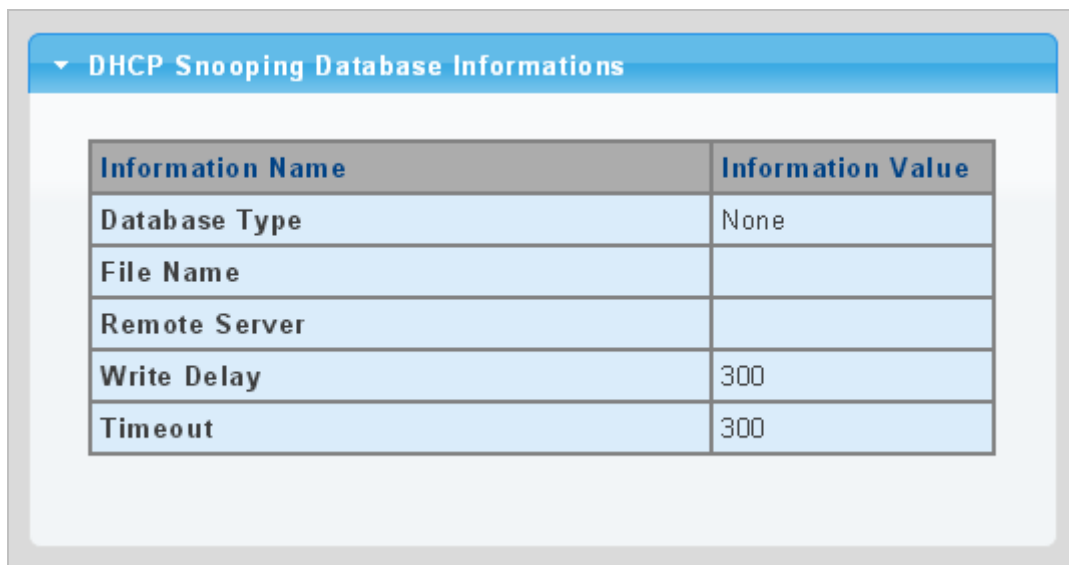
Figure 4-9-43 DHCP Snooping Database Information Page Screenshot
