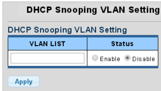
Figure 4-9-37 DHCP Snooping VLAN Setting Page Screenshot
