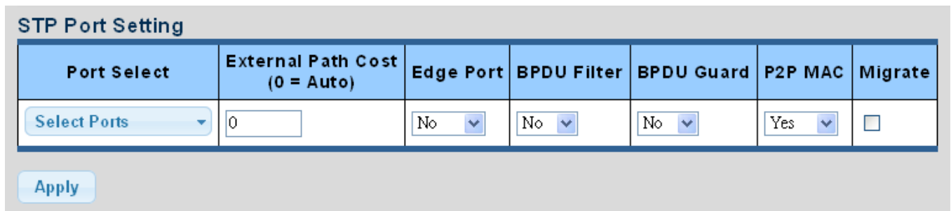
Figure 4-6-6 STP Port Configuration Page Screenshot
