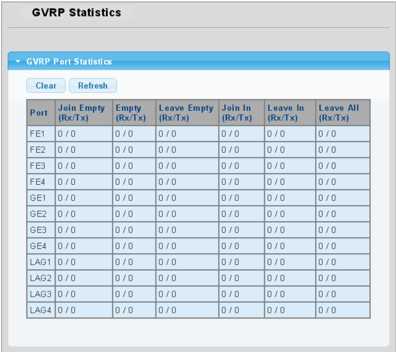
Figure 4-5-18 GVRP Port Statistics Page Screenshot
