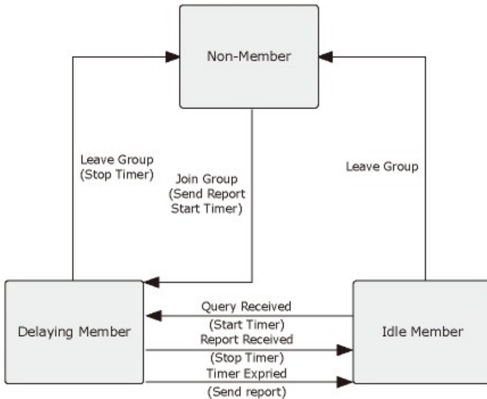
Figure 4-7-6 IGMP State Transitions
