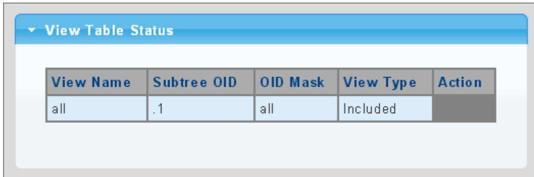
Figure 4-2-23 SNMP View Table Status Page Screenshot
