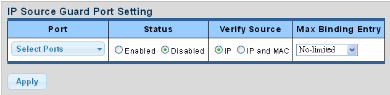
Figure 4-9-61 IP Source Guard Port Setting Page Screenshot
