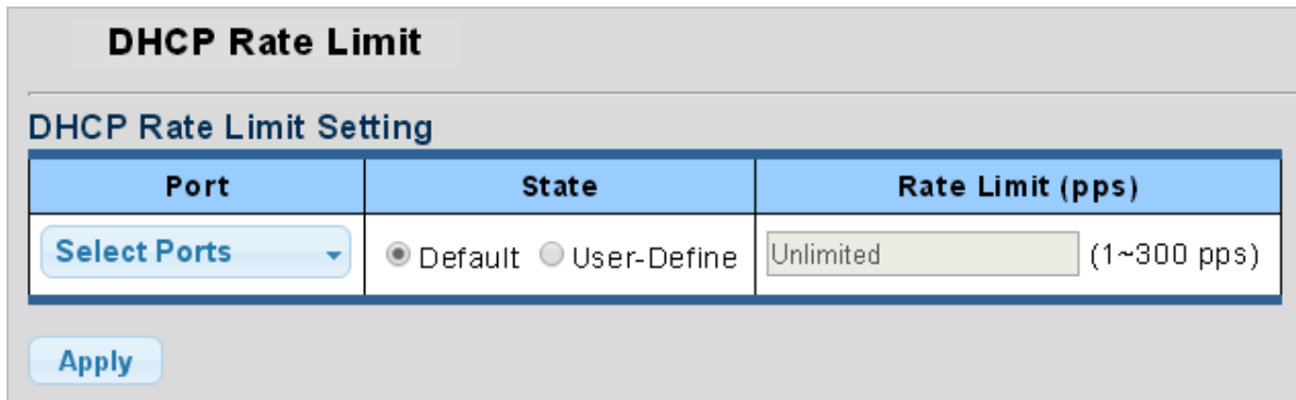
Figure 4-9-44 DHCP Rate Limit Setting Page Screenshot
