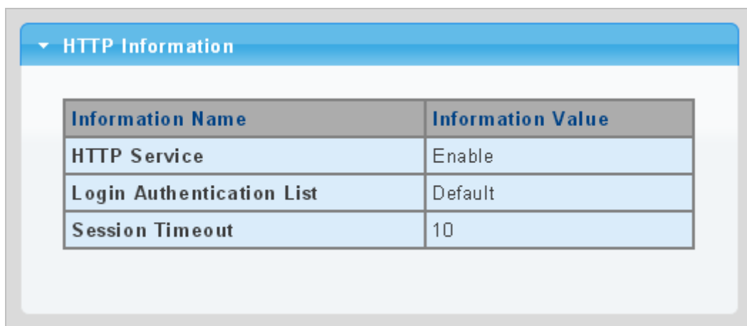
Figure 4-9-26 HTTP Information Page Screenshot8
