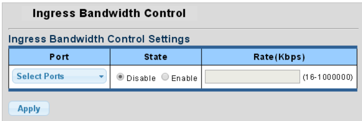
Figure 4-8-16 Ingress Bandwidth Control Settings Page Screenshot
