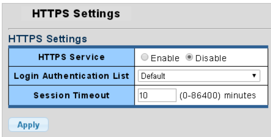
Figure 4-9-29 HTTPS Settings Page Screenshot
