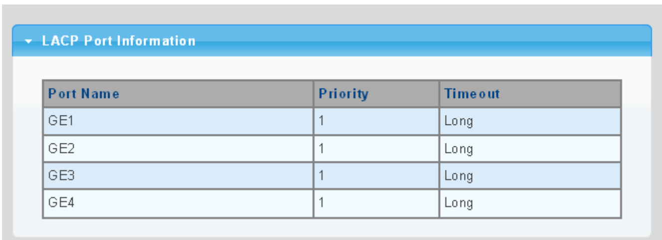
Figure 4-4-11 LACP Port Information Page Screenshot
