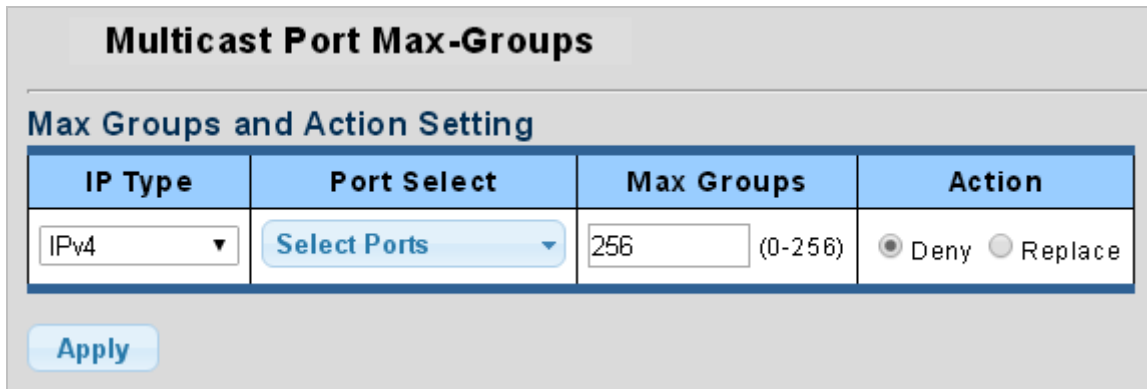
Figure 4-7-34 Max Groups and Action Setting Page Screenshot
