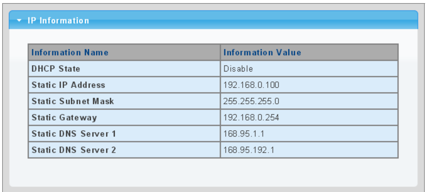
Figure 4-2-3 IP Information Page Screenshot
